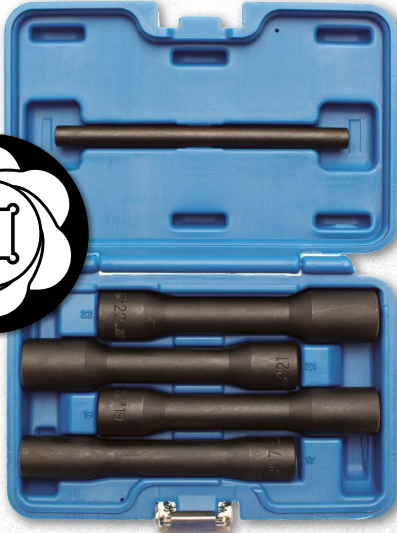
Twist Socket Set (Spiral Profile) / Screw Extractor, deep | 12.5 mm (1/2") Drive | 17 - 22 mm | 5 pcs.
